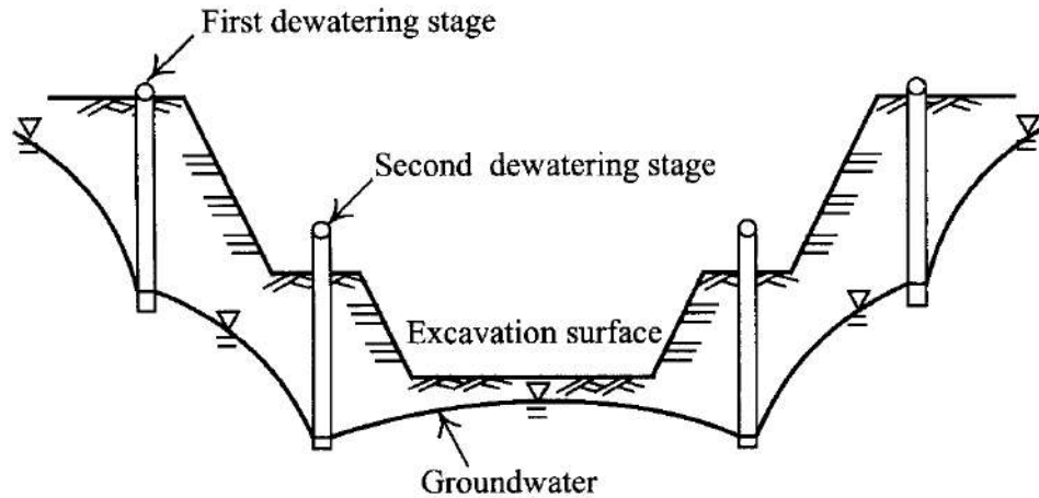
Two Stage Well Point Systems
